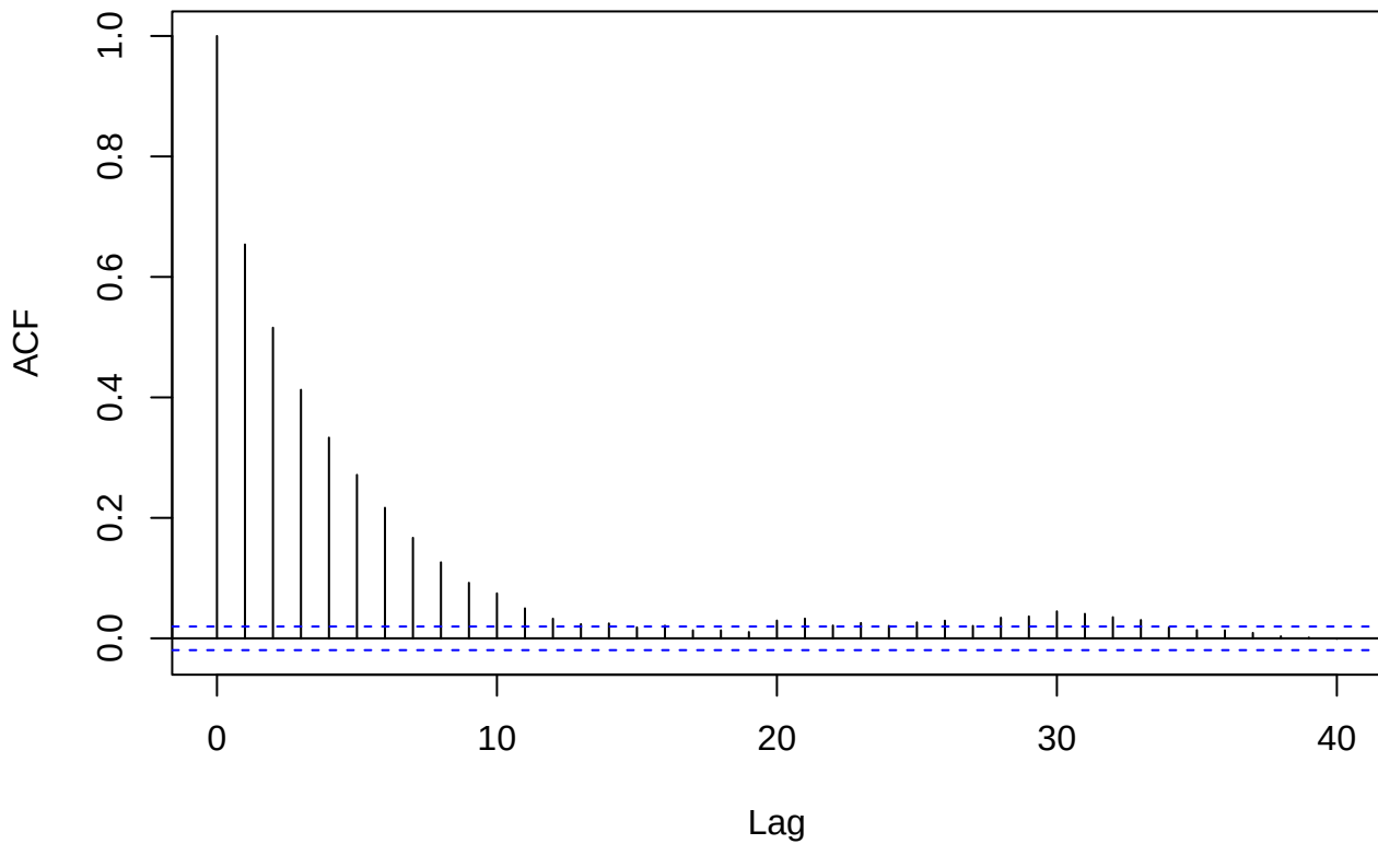
Series of_gibbs_10$means[2, ]
